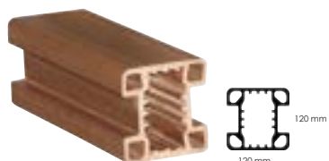
PROFILE FP120120 FENCING POST 120 x 120 W 120mm x H 120mm
