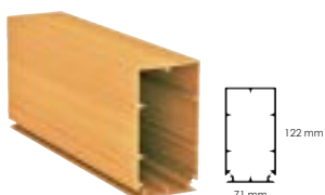
PROFILE PC12271 POST COVER 122 x 71 W 122mm x H 71mm
