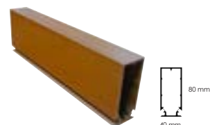
PROFILE PC08040 POST COVER 80 x 40 W 80mm x H 40mm
