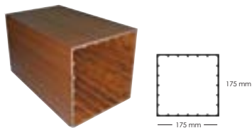
PROFILE PS175175 POST SUPPORT 175 x 175 W 175mm x H 175mm
