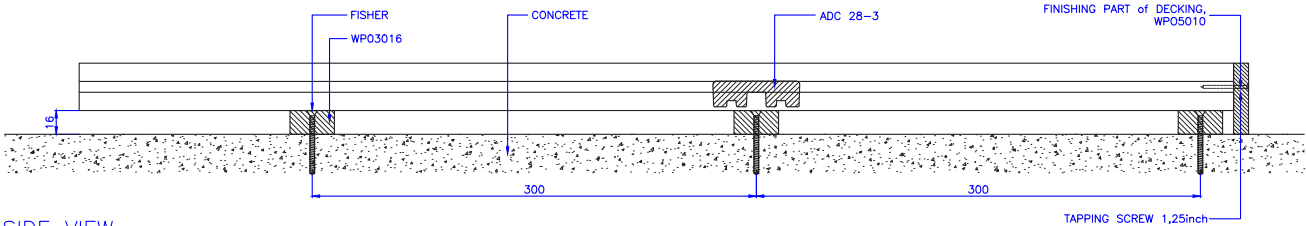
SIDE VIEW
