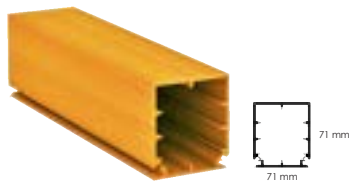
PROFILE PC07171 POST COVER 71 x 71 W 71mm x H 71mm
