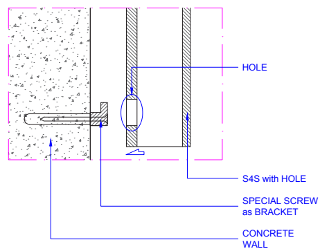
DETAIL A 01
